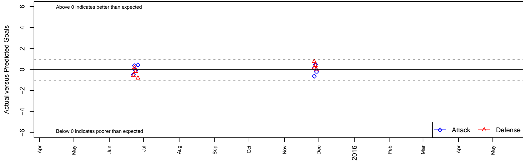
Pride SC 99 Predators G98 Dots are actual minus expected GF (blue circles) and GA (red triangles). Blue line is smoothed change in attack strength. Red is smoothed change in defense strength.
